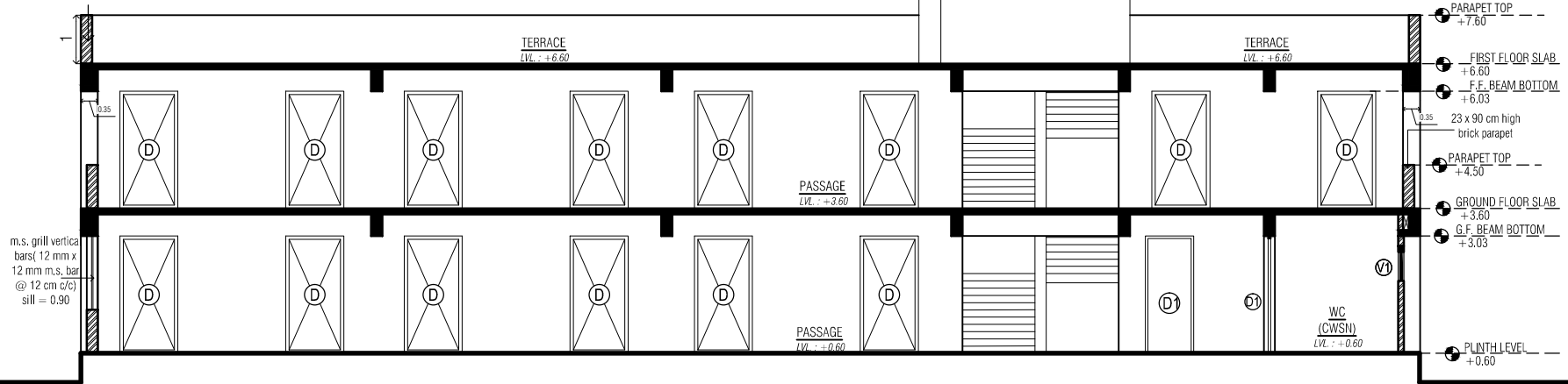
SECTION -2-2
