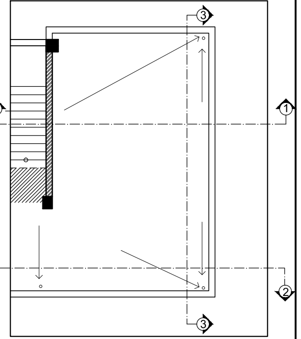
TERRACE PLAN
