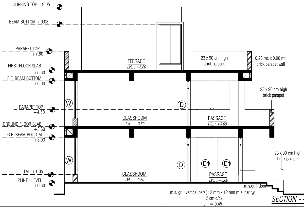
SECTION - 3-3
